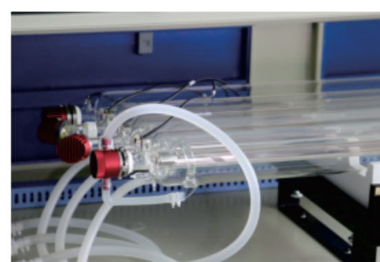
激光管 Laser Tube
